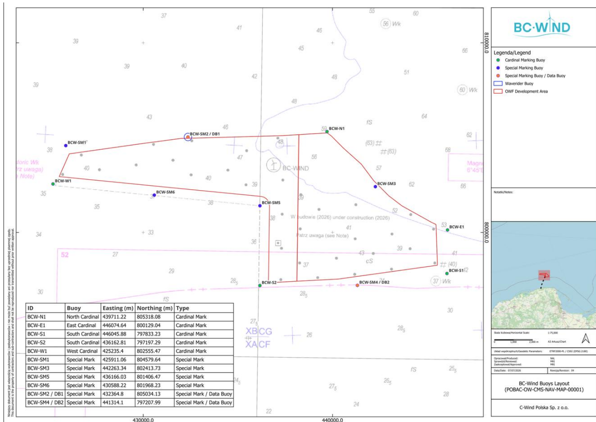
Pic 2 Demarcation buoys and data buoys chart
